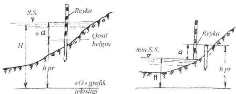
2.3-rasm. Suv sathini nol grafikka nisbatan o'lchash a – musbat sanoq ( +a ); b – manfiy sanoq ( -a ).
